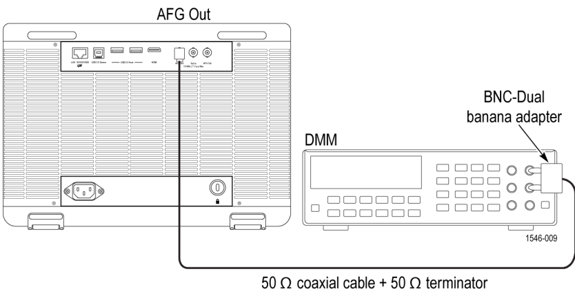
Figure 4: Amplitude test
