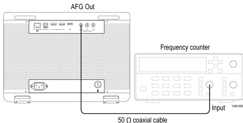
Figure 1: Frequency/period test
