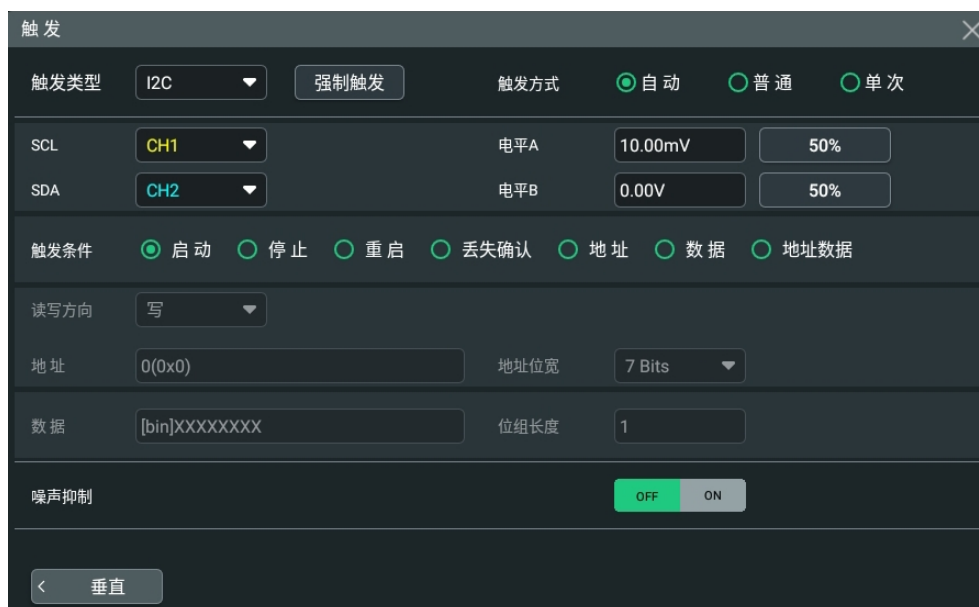
图 8.27 I2C 触发配置菜单
