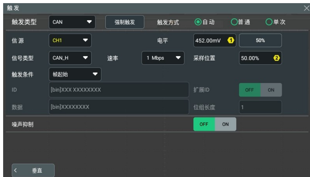
图 8.33 CAN 触发配置菜单
